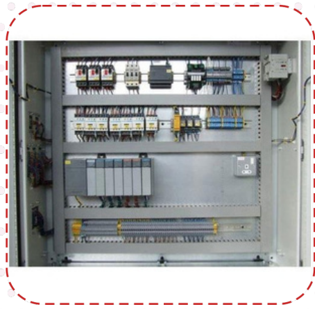
PLC CONTROL PANEL PROGRAMMABLE LOGIC CONTROLLER PANEL
